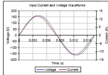
Input AC Current Waveform (THD = 6.04%, 50% Load)
