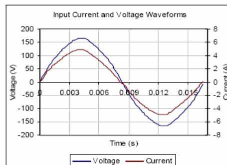
Input AC Current Waveform ( I_{THD} = 4.1\% at 100% Load)
